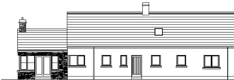
PROPOSED REAR ELEVATION 1/100.
