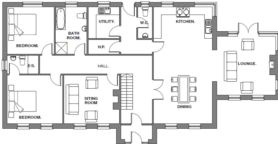
PROPOSED GROUND FLOOR LAYOUT 1/100.
